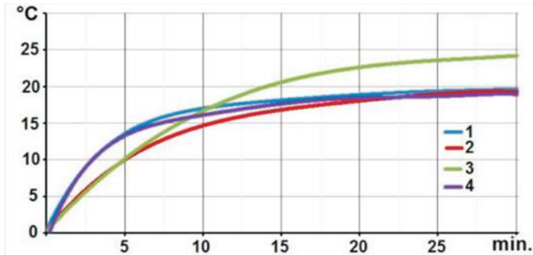
Chart of the terminal temperature rise for a 16A intensity depending on the model and their protection
